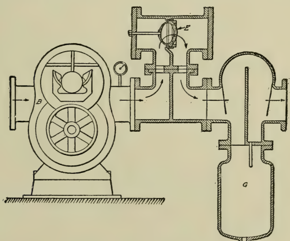
FIG. 71.—Smith Tar Extractor.
